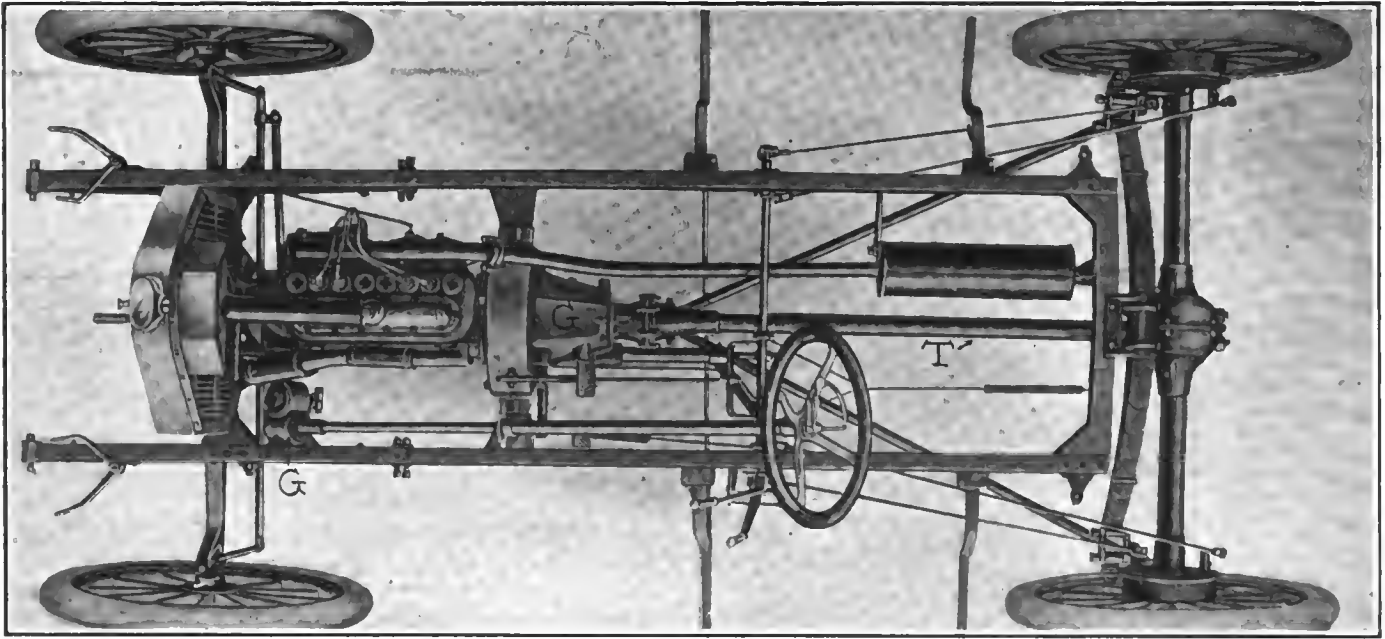
Fig. 1—Plan view of the 1912 Krit model "A" runabout chassis
